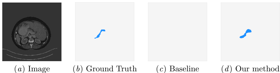
Figure 2: Qualitative results
